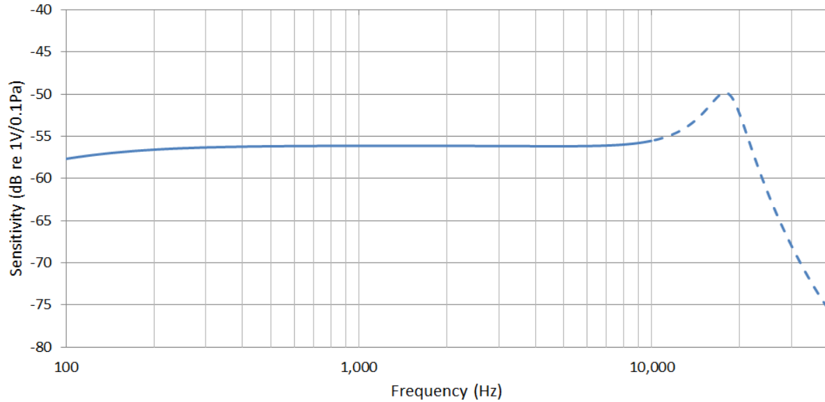
Figure 1: Typical frequency response measured in a pressure cavity under nominal conditions (Table 1). Response above 10 kHz is typical in free field and not measured in the pressure cavity.
