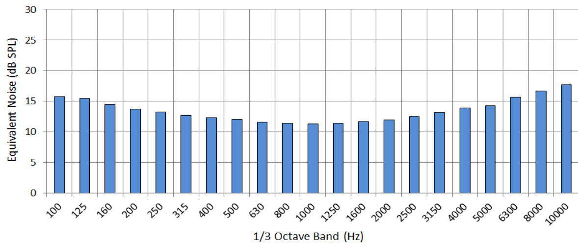
Figure 2: Typical Equivalent Noise under nominal conditions (Table 1)
